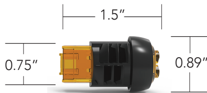
Molded connector style
